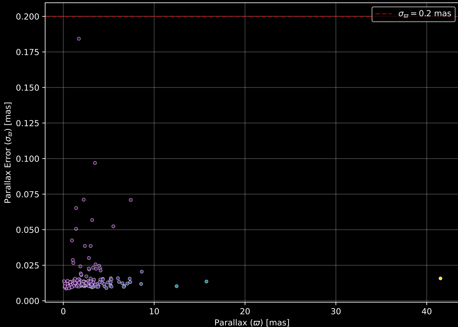
APOGEE DR17 Field: [CVZ_OB21_btx] Parallax Quality (n= 175)
