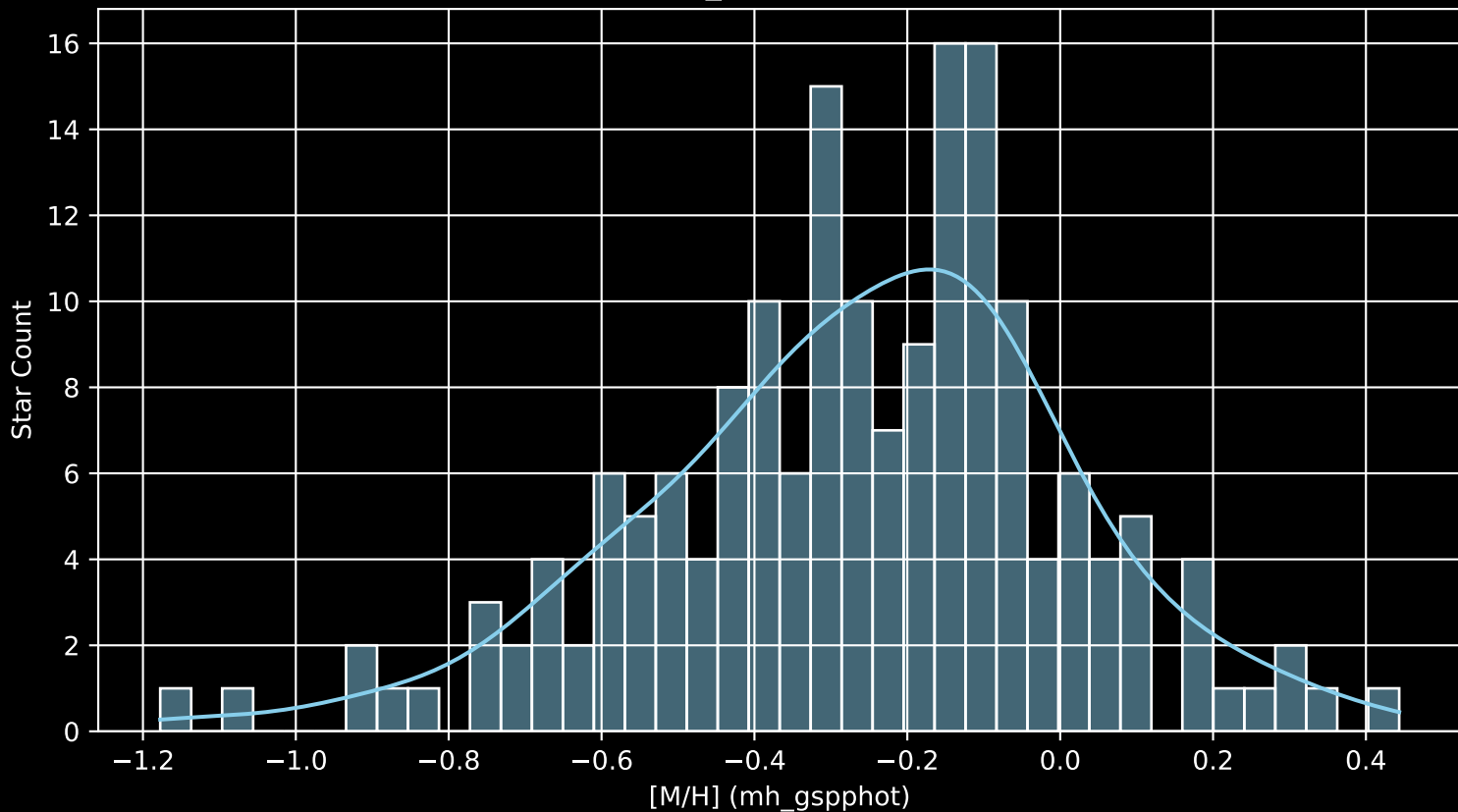
APOGEE DR17 Field: [CVZ_OB21_btx [M/H] (mh_gspphot) (n= 174)
