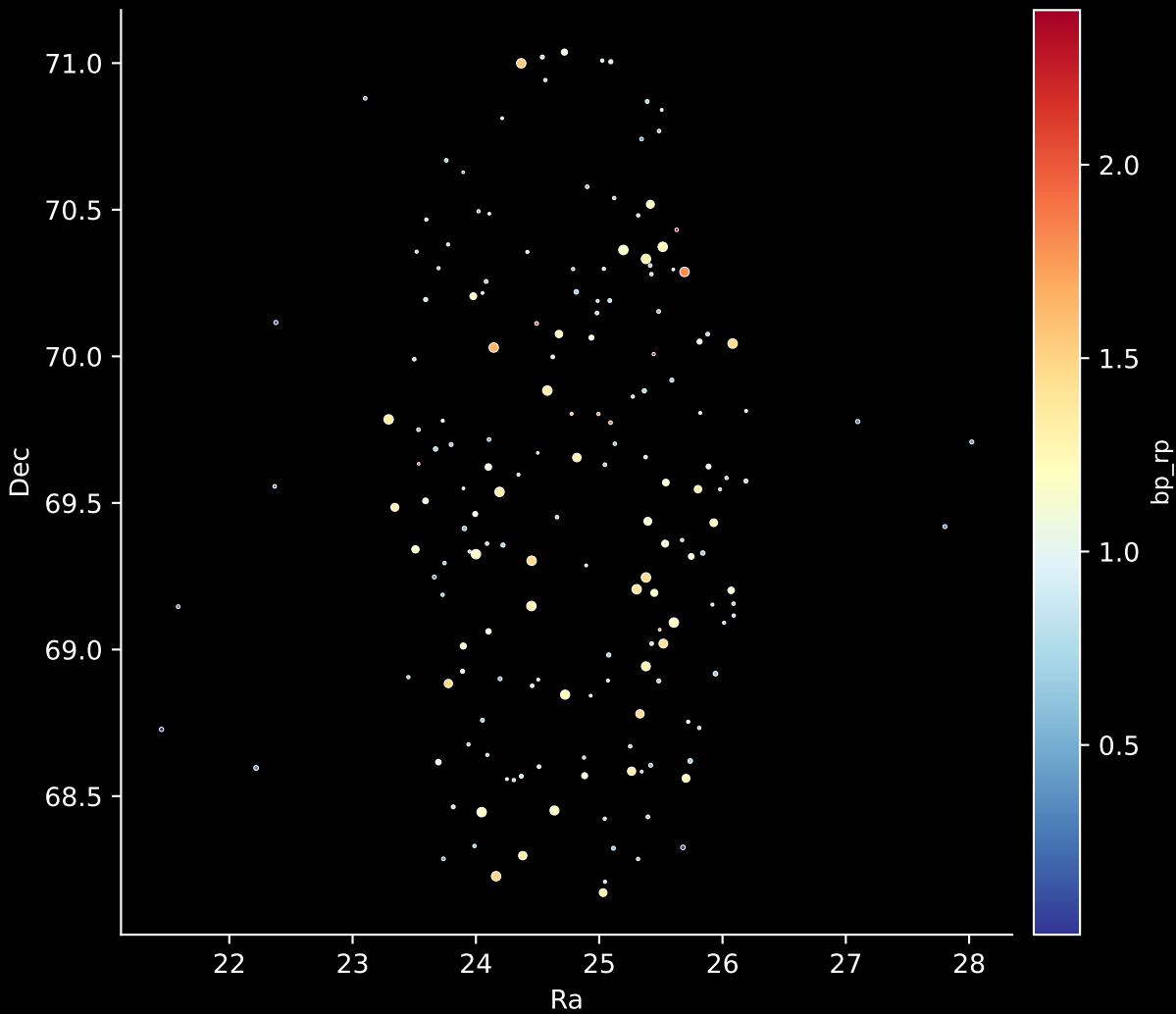
APOGEE DR17 Field: [CVZ_OB21_btx] Stars: 175
