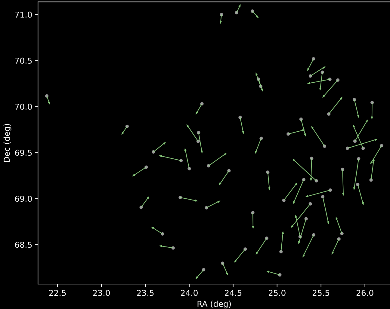
APOGEE DR17 Cluster 5 Proper Motion Vectors (n=62)
