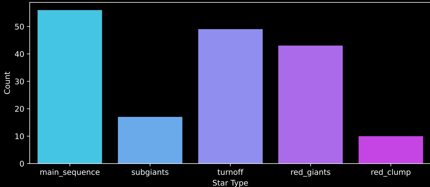
APOGEE DR17 Field: [CVZ_OB21_btx] Count plot of Star Type
