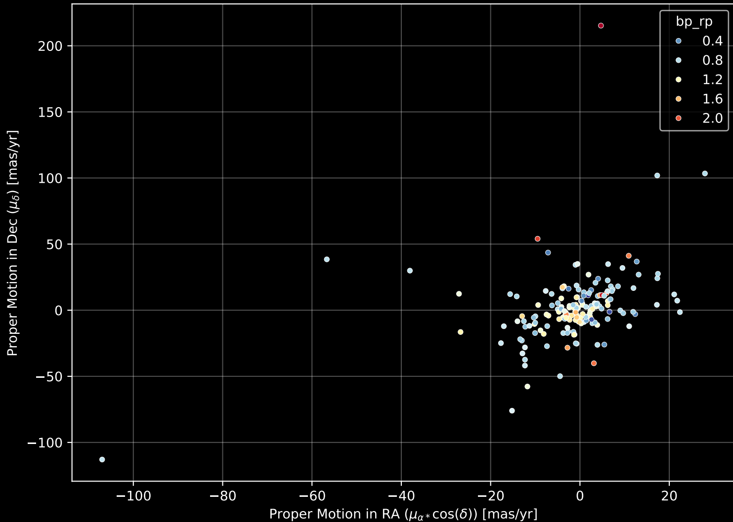
APOGEE DR17 Field: [CVZ_OB21_btx] Proper Motion Diagram (n= 175)
