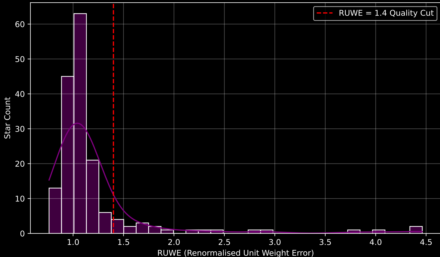
GAPOGEE DR17 Field [CVZ_OB21_btx] RUWE Distribution (n= 169)
